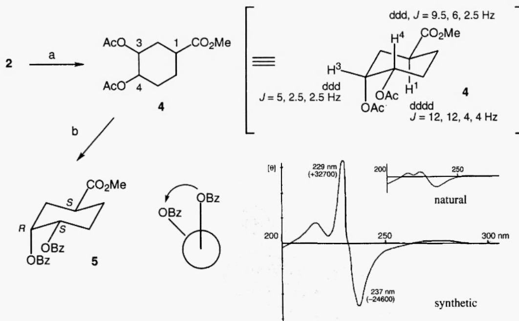
Scheme 1. Derivation of 2 and CD spectra of natural and synthetic 5 .
