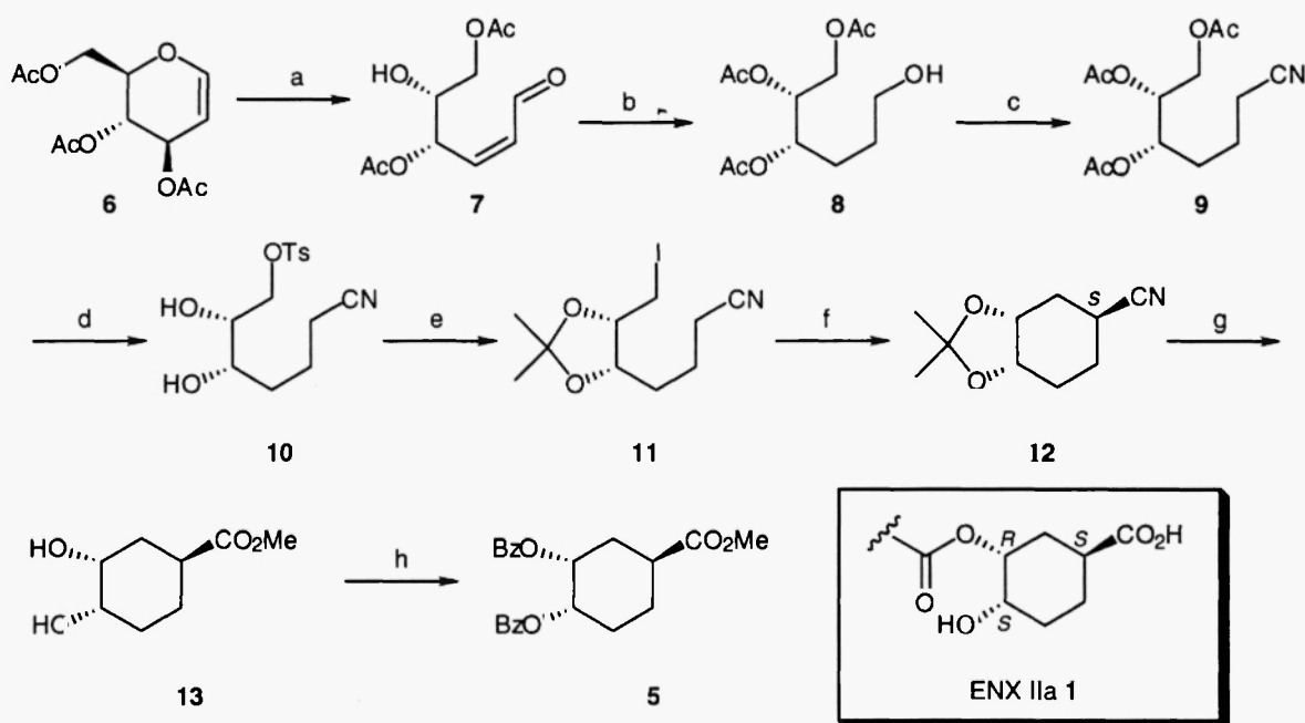
Scheme 2. Synthesis of 5 from tri- O -acetyl-D-glucal 6 .
