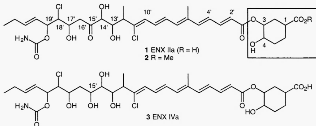
Fig. 1. Enacyloxin Ila 1 and its derivatives.
